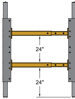
End View Sectional corner post with adjustable struts
